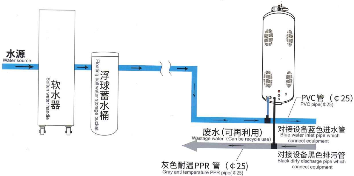
推荐安装示意图 Recommend installation diagrammatic sketch
